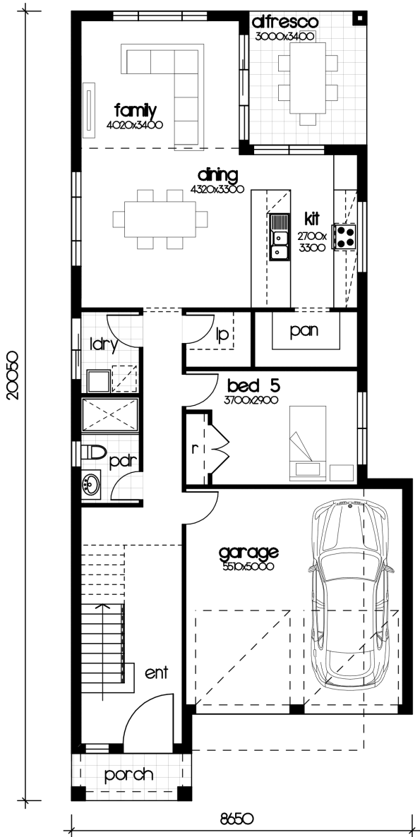
GROUND FLOOR PLAN RUBY 28 (5 BED OPTION) - EXECUTIVE FACADE - RH
