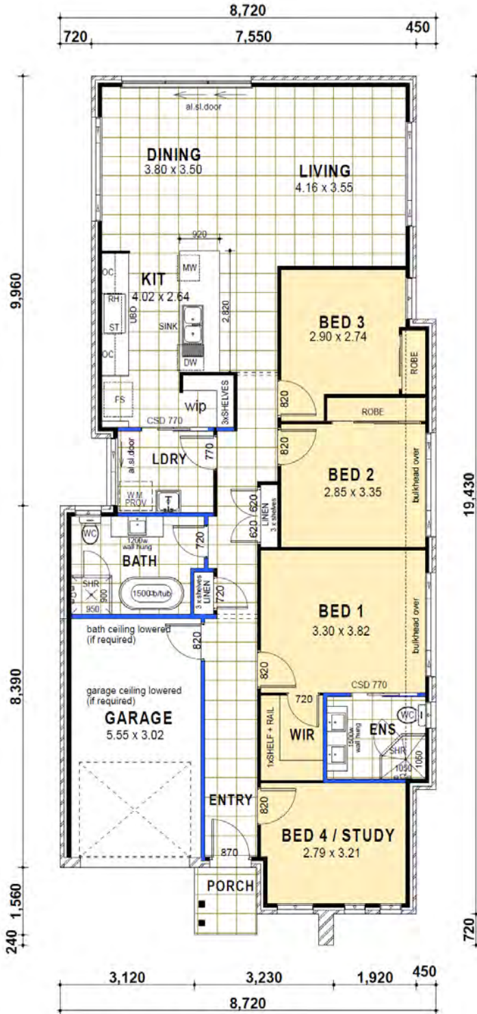
floor plan
